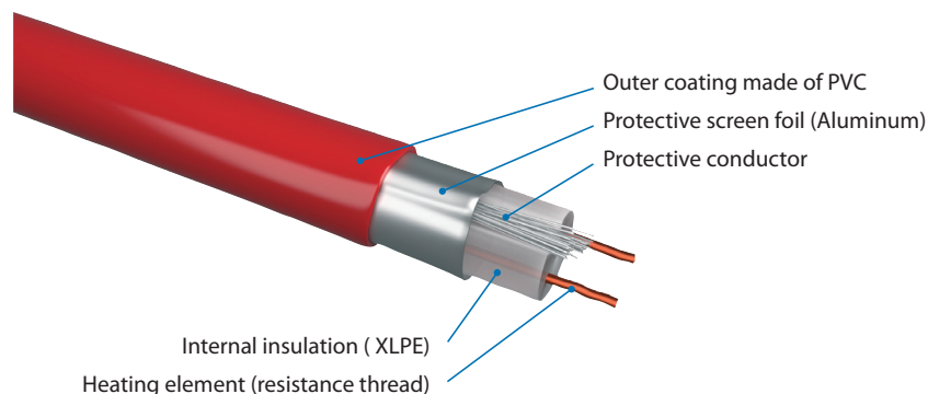
DEVIflex™ heating cable construction
