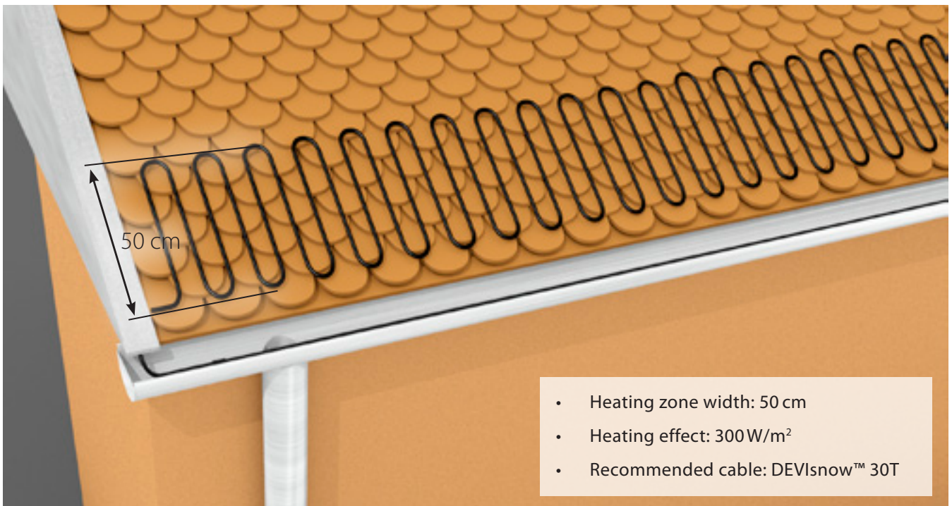
Roof edges and gutter with heating installation.
